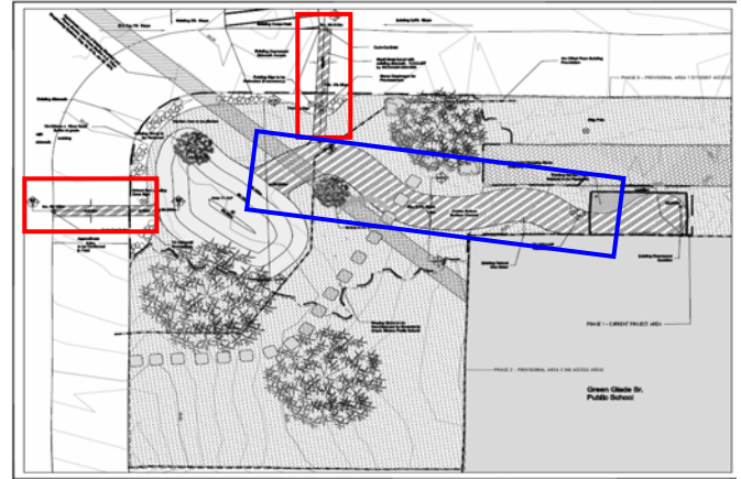
Rain garden site plan
