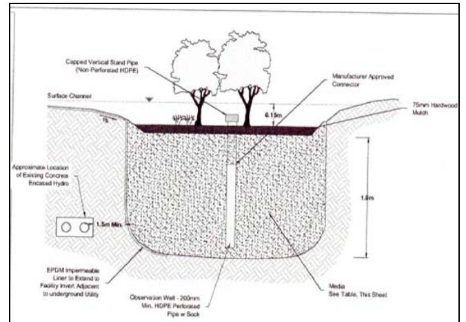
Cross section of the rain garden
